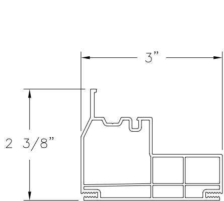
MAIN FRAME (CH9201A) EXTRUDED RIGID PVC
