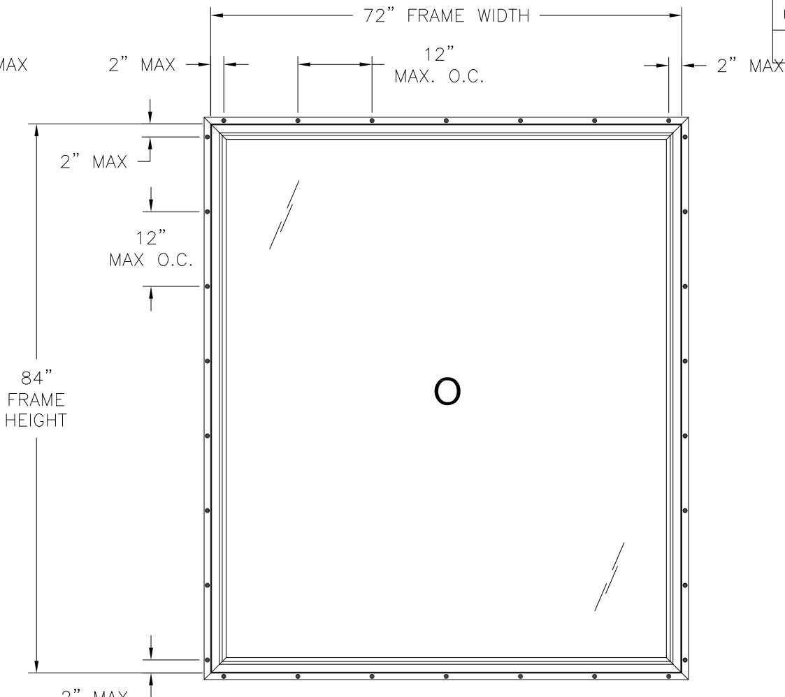
200/275 VINYL PICTURE WINDOW EXTERIOR VIEW FIN INSTALLATION
