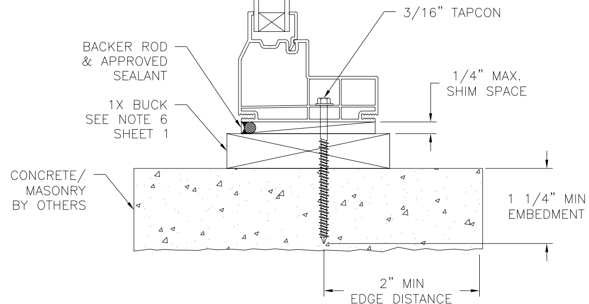
VERTICAL CROSS SECTION CONCRETE/MASONRY WITH 1X BUCK INSTALLATION FOR CONCRETE/MASONRY INSTALLATION WITHOUT 1X BUCK REFER TO JAMB INSTALLATION DETAILS
