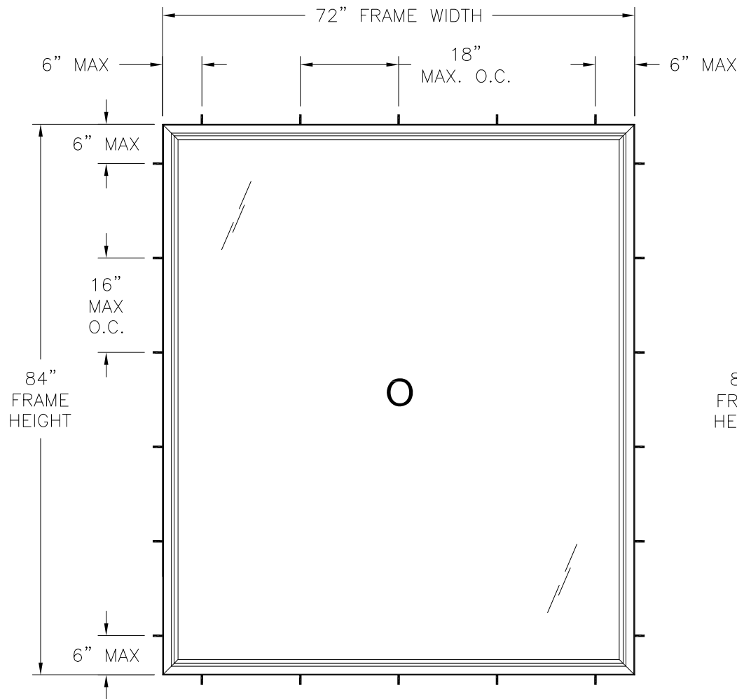
200/275 VINYL PICTURE WINDOW EXTERIOR VIEW FRAME INSTALLATION
